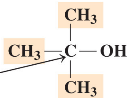
Tertiary (3°) alcohol
