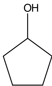
Cyclopentanol
