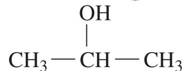
Isopropyl Alcohol
