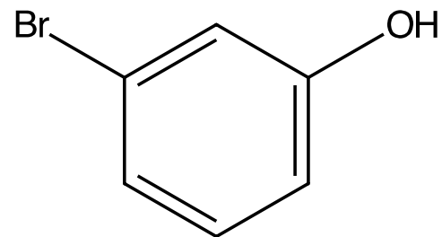
3-Bromophenol
