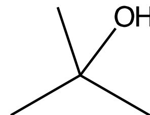
Tertiary (3°) alcohol
