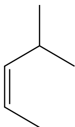
cis -4-Methyl-2-pentene
