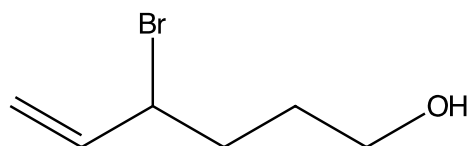
4-Bromo-5-hexen-1-ol
