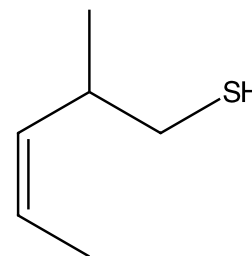
cis -2-Methyl-3-pentene-1-thiol
