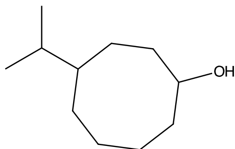
4-Isopropylcyclooctanol
