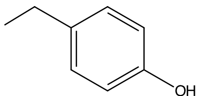
4-ethylphenol
