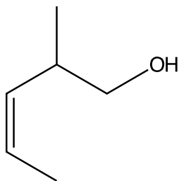
cis -2-Methyl-3-penten-1-ol
