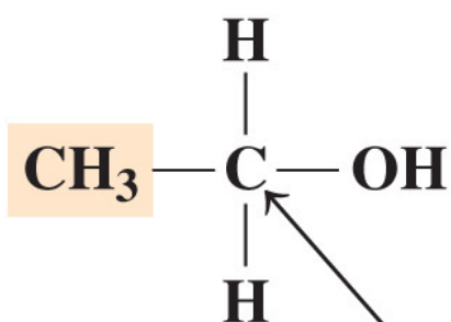
Primary (1°) alcohol
