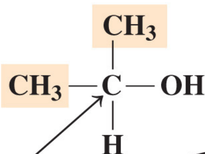
Secondary (2°) alcohol
